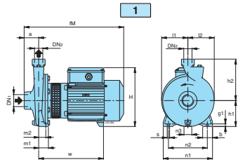
Standard construction
